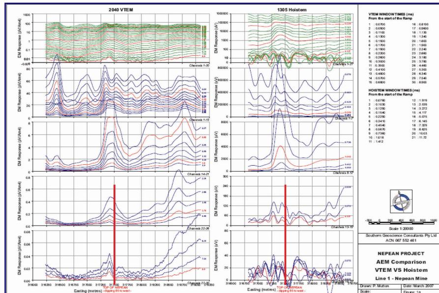
Figure 1. Comparison of VTEM data on the left panel with Hoistem data on the right panel over "Line 1 - Nepean Mine".
