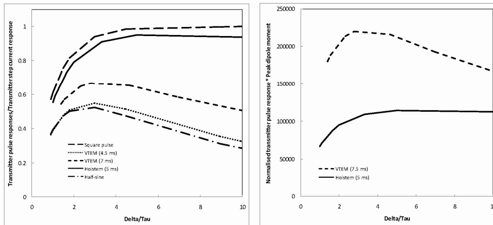
Figure 2 (a) Ratio of the response for a selected transmitter pulse to that of the step current as a function of \Delta/\tau . (extended from Liu 1998). (b) Normalised VTEM and Hoistem responses multiplied with the respective peak dipole moments to give the effective system responses.
