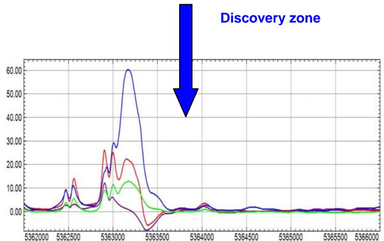
Aerodat coax profiles, line 10240
