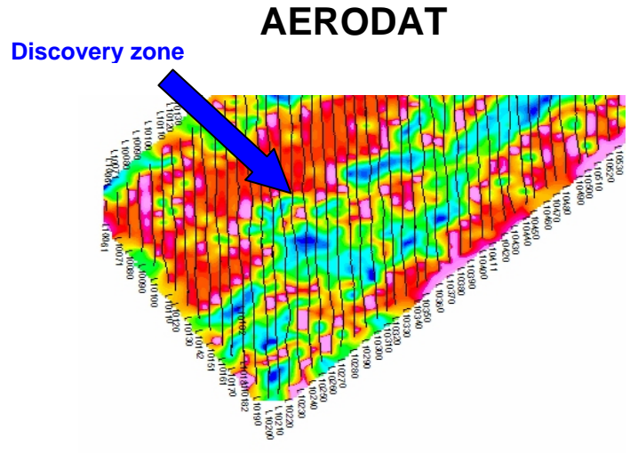
Aerodat Resistivity Map showing no clear definition
